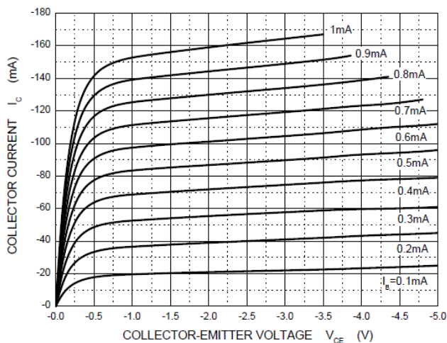
Static Characteristic
