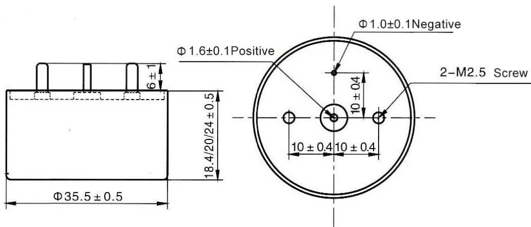
Φ35.5x18.4/20/24 Layout
